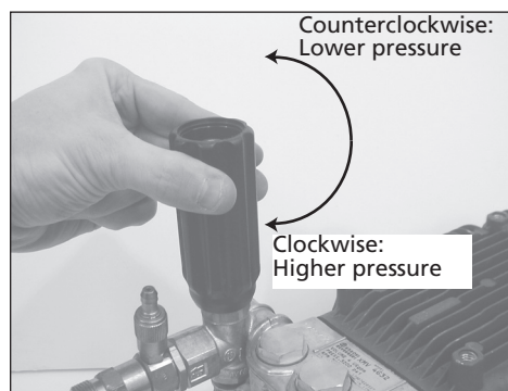
Figure 11 - Camshaft pump pressure adjustment
