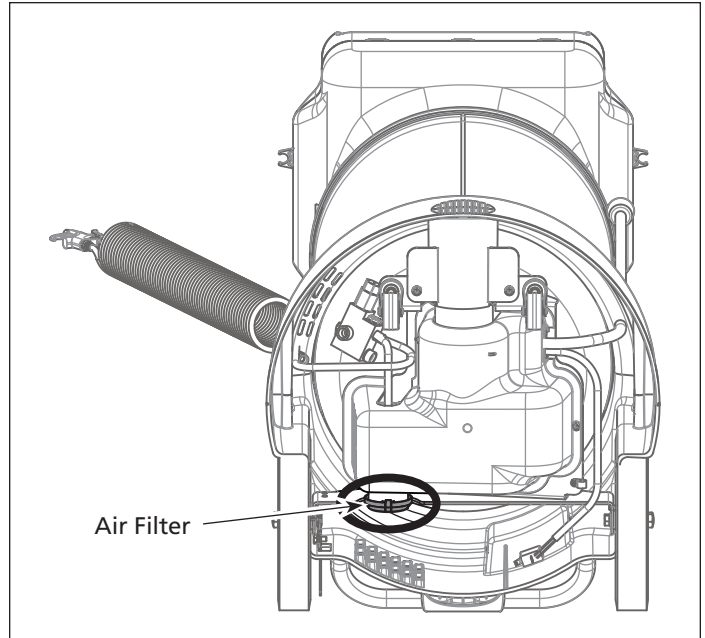
Figure 19 - Air Filter
