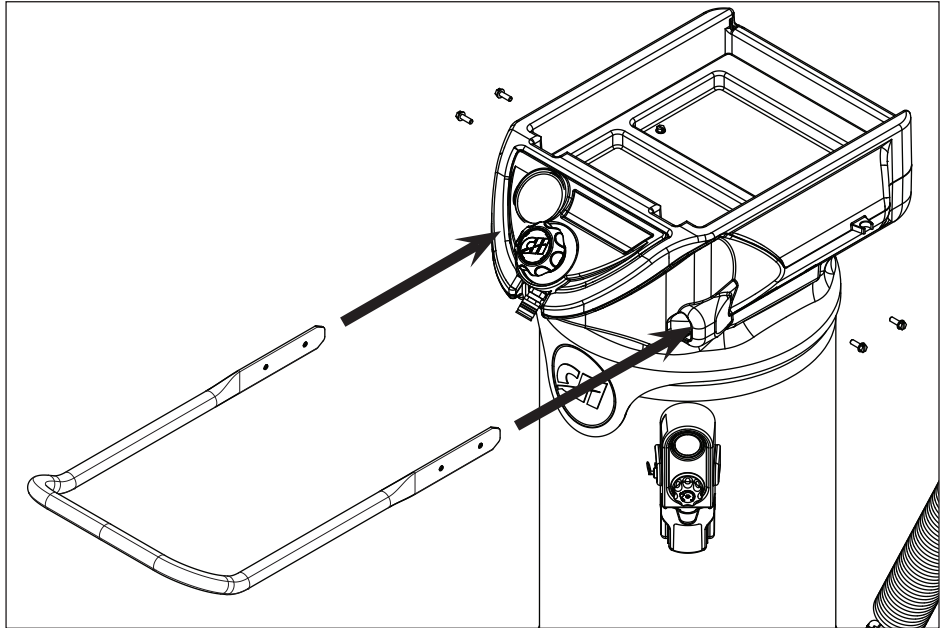
Figure 9 - Handle assembly
