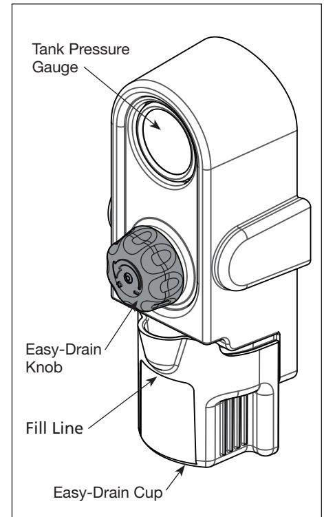
Figure 18 - Draining tank
