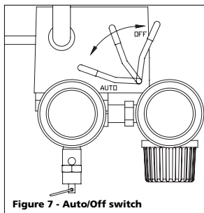
Figure 7 - Auto/Off switch
