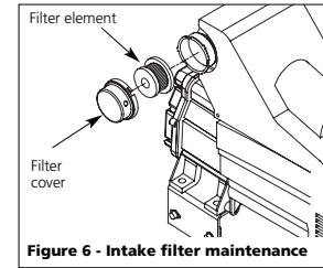
Figure 6 - Intake filter maintenance
