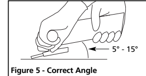
Figure 5 - Correct Angle
