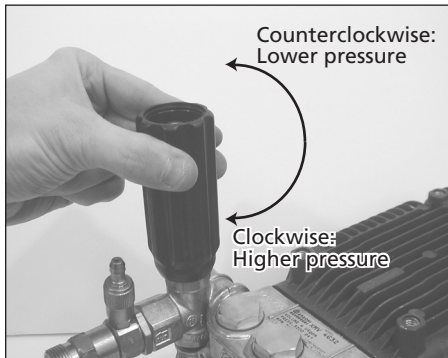
Figure 11 - Camshaft pump pressure adjustment
