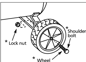
Figure 2 - Wheel Assembly
