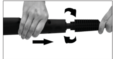
Figure 19 - Gun/lance connection
