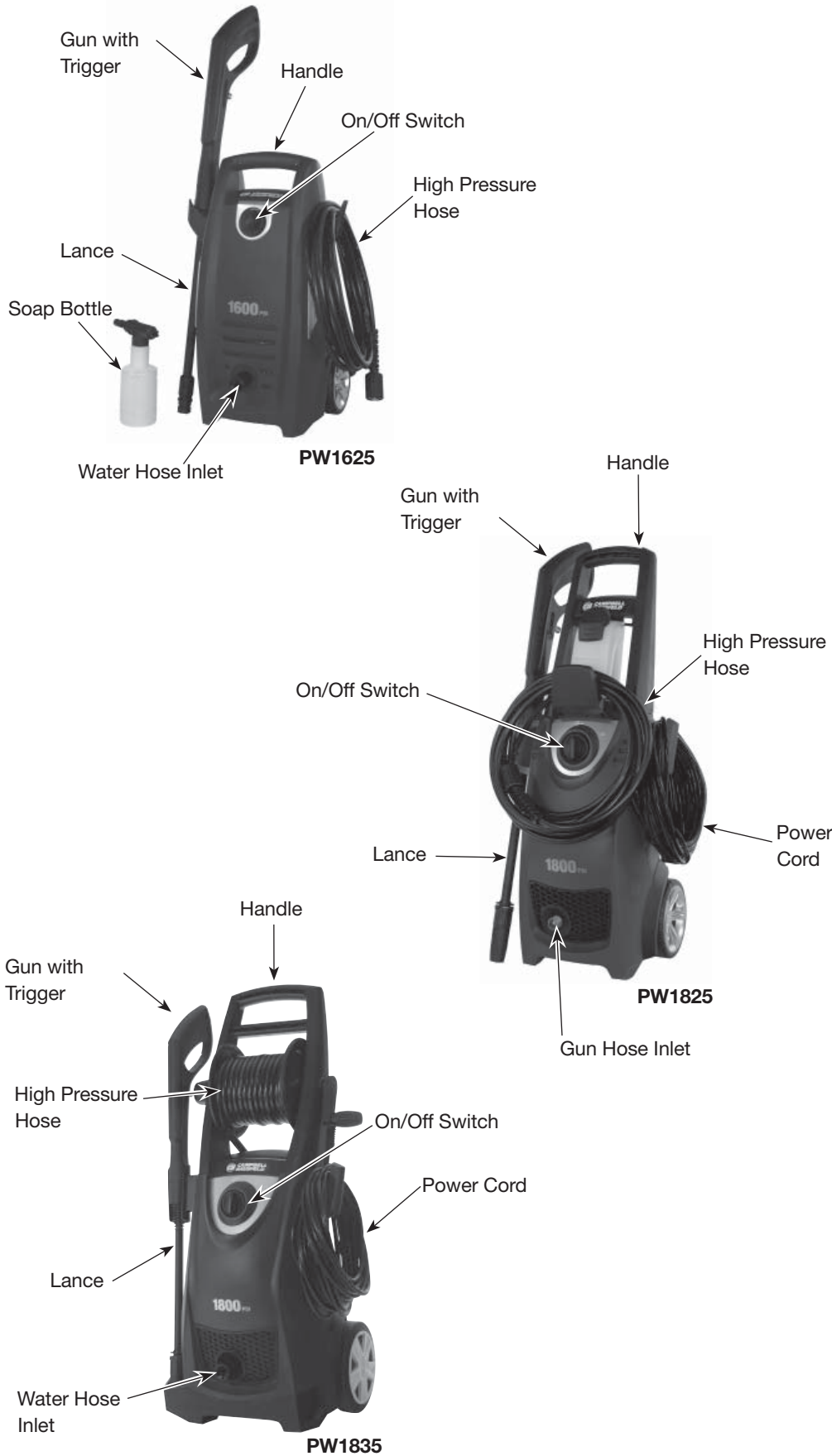
Figure 6 - Components of the Pressure Washer
