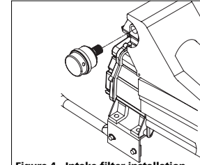
Figure 4 - Intake filter installation
