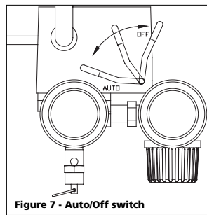
Figure 7 - Auto/Off switch
