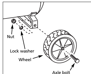
Figure 2 - Wheel Assembly
