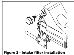
Figure 2 - Intake filter installation
