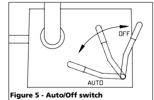
Figure 5 - Auto/Off switch
