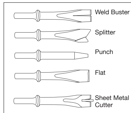
Figure 5 - Hammer Bits
