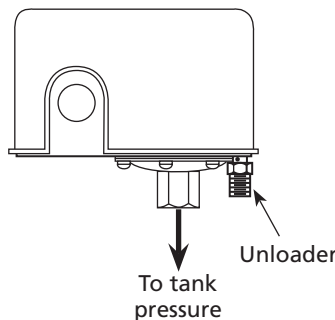
Figure 7 - Pressure Switch
