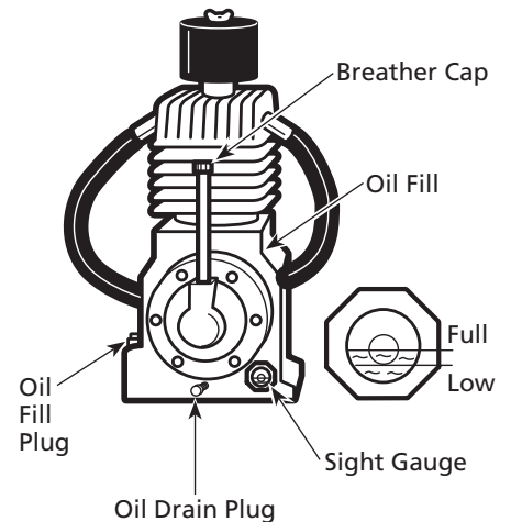
Figure 5 - Oil Fill Diagrams
