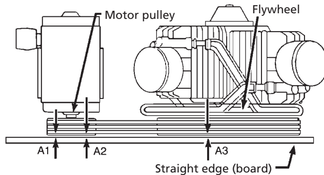
Figure 9 - Top view
