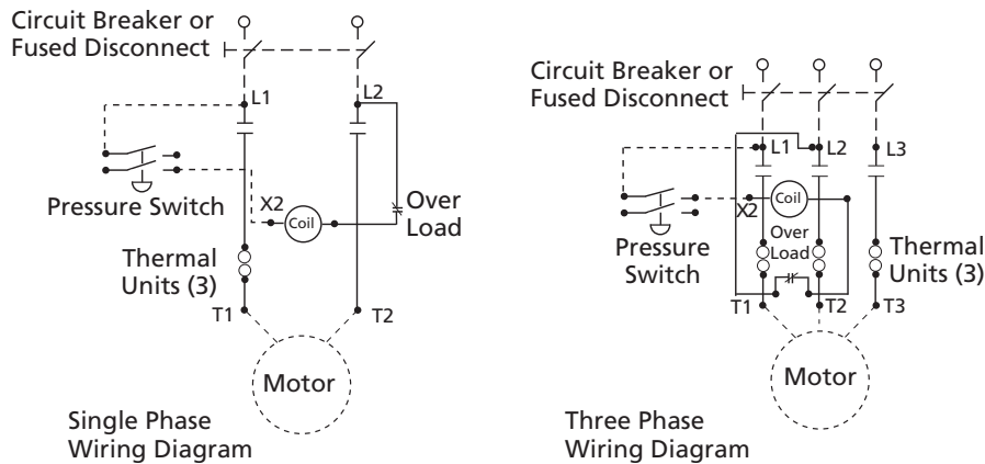
Figure 4 - For Motor Frame Sizes 184T, 215T, 254T or 284T. Refer to Motor Nameplate
