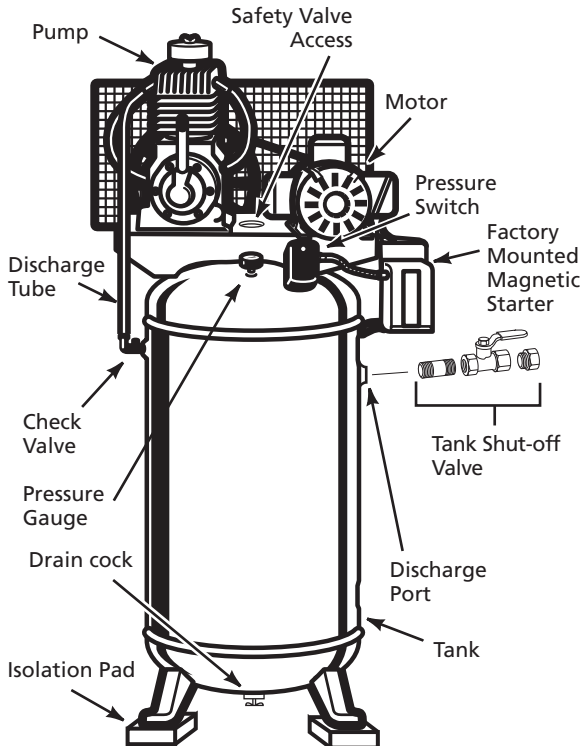
Figure 1 - Vertical Unit Identification
