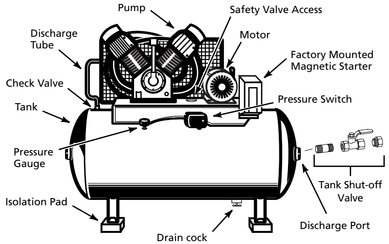
Figure 2 - Horizontal Unit Identification
