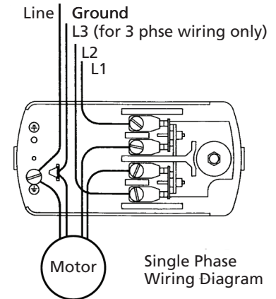
Figure 3 - For Motor Frame Sizes R56HZ, Y56Y or L143T. Refer to Motor Nameplate
