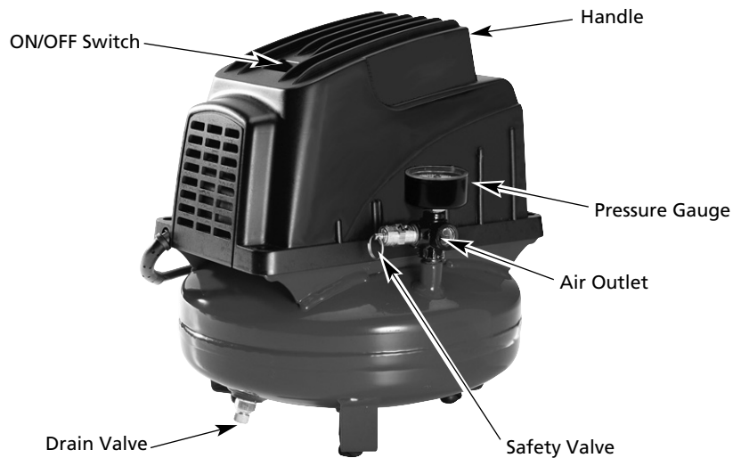
Figure 2 - Unit Identification
