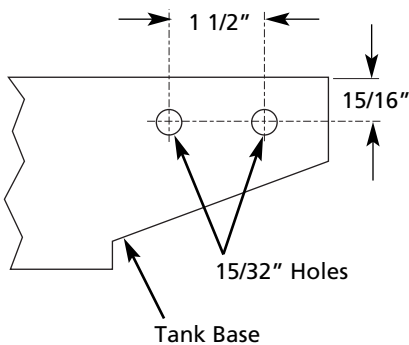
Figure 2 - Drilled holes
